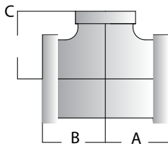
Reducing Tee
